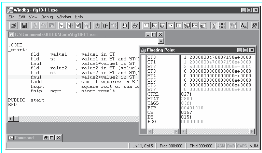
Figure 10.12 Execution of floating-point example
