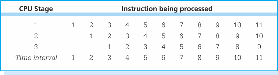
Figure 5.11 Instructions in a pipeline
